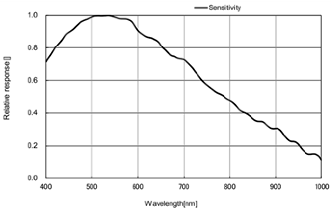
MER2-1220-32U3M 光谱曲线
